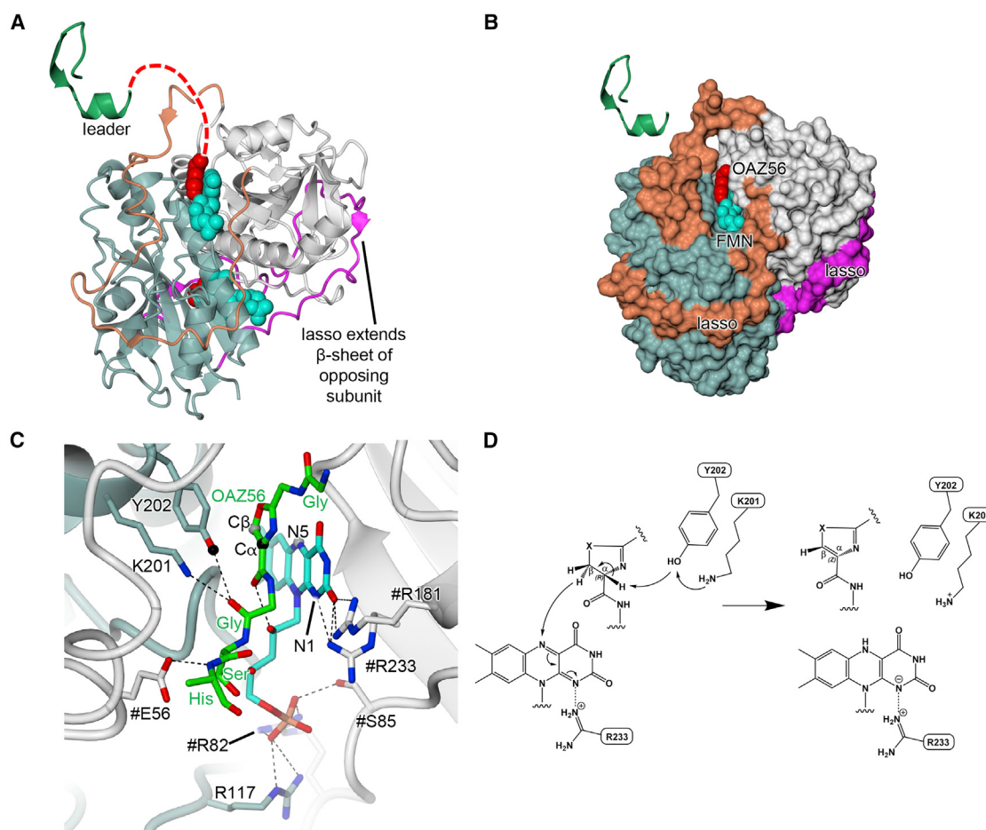
Figure 6. The Structure and Mechanism of the Dehydrogenase MccB
