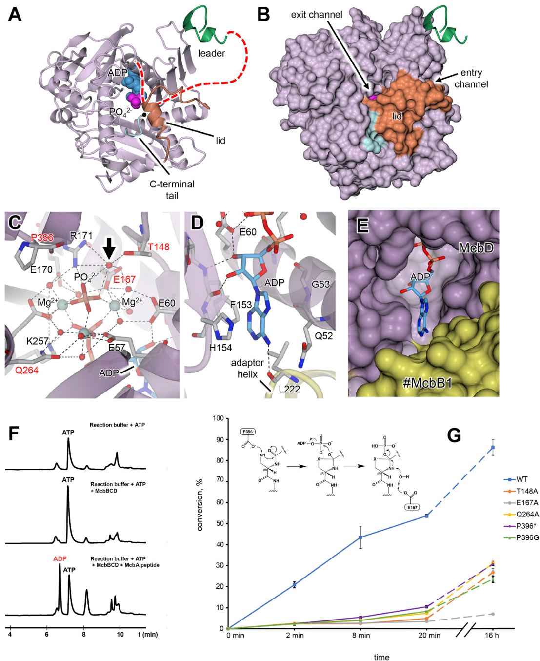
Figure 5. The Structure and Mechanism of the Heterocyclase McbD
