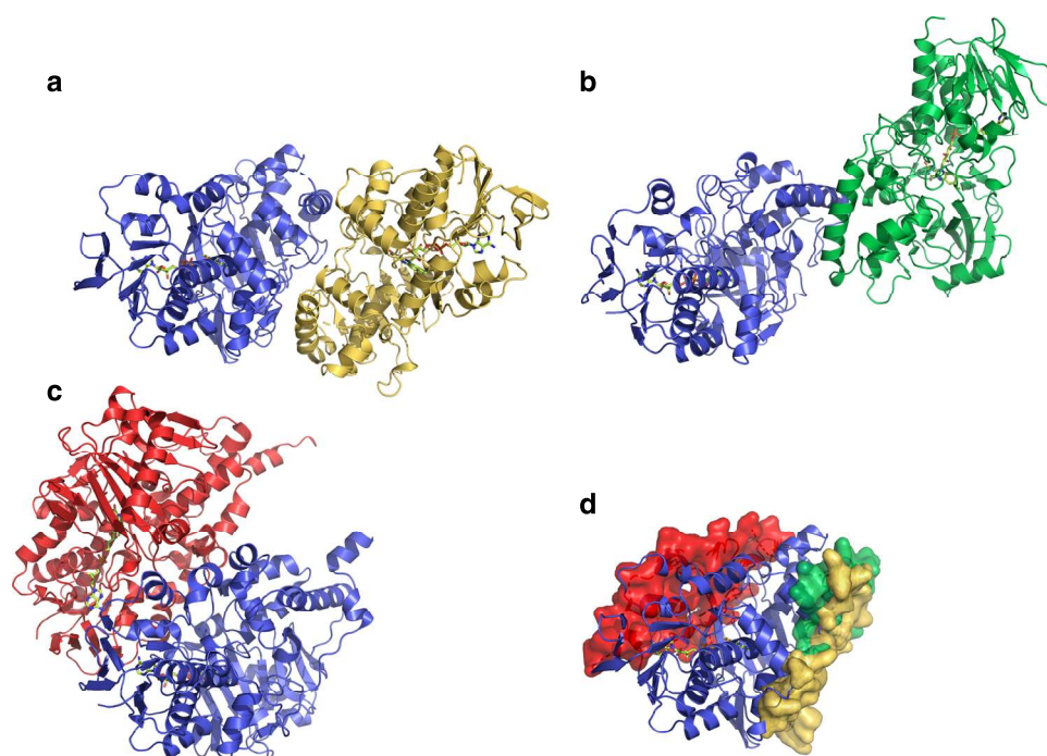
Fig. 5 Alternate homodimerization mode of LkcE relative to hMAO B and 6HDNO. a Homodimeric structure of LkcE. The dimer is superimposed on one monomer of LkcE (in blue in a ), in the same orientation. b Homodimerization mode of 6HDNO. The dimer is superimposed on a monomer of LkcE. c Homodimerization mode of hMAO B. Again, the dimer has been superimposed on a monomer of LkcE. d Interaction surface between the two monomers in LkcE (yellow), hMAO B (red), and 6HDNO (green), relative to a monomer of LkcE. This analysis clearly shows that the mode of homodimerization of LkcE, as well as its overall quaternary organization, differ from these two homologs
